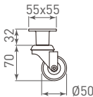
ZPT-AKE50ABN-220BNB (with brake)
